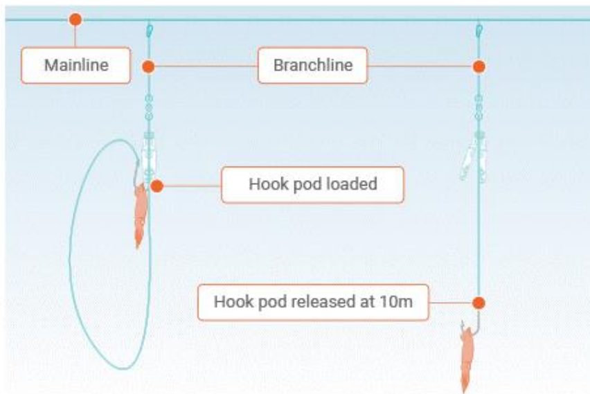
Figure 8. Schematic showing how the hookpod works to protect baited hooks and open at depth. (Source: B. Ingram, Hookpod Ltd).
