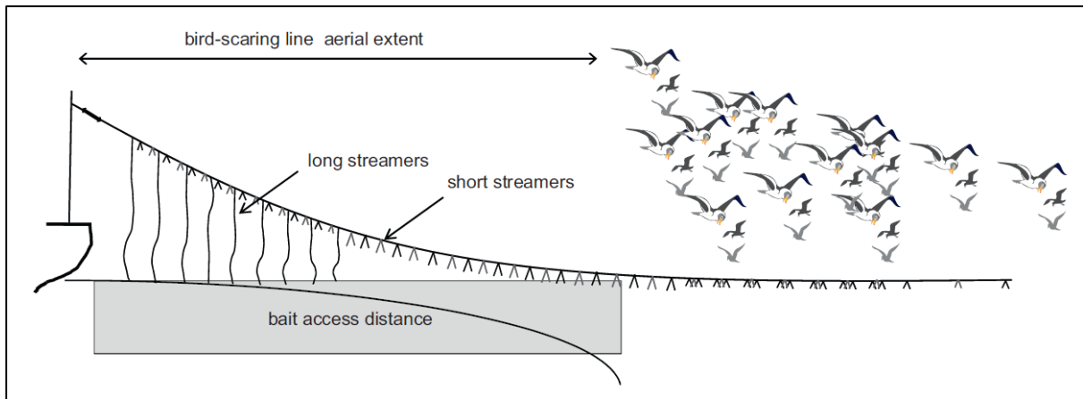
Figure 1. Schematic diagram of a bird-scaring line deployed astern a pelagic longline vessel. (Modified from Melvin et al. 2014).
