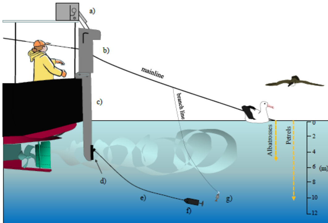
Figure 9. Schematic of the underwater bait setter recognised as best practice by the Agreement on the Conservation of Albatrosses and Petrels (not to scale). Components parts are: (a) winch assembly, (b) head section of the track assembly, (c) the track attached to the vessel transom, (d) capsule docking cart, (e) Spectra rope connecting the capsule to the recovery motor winch, (f) capsule with bait door fully extended and (g) baited hook following release from the capsule. The system's control unit is located in the wheelhouse and operated by the skipper. Dive depths of the main seabird groups are indicated on the right. The curved shapes above the capsule depict water thrust from the propeller. (Source: Robertson et al. 2015).
