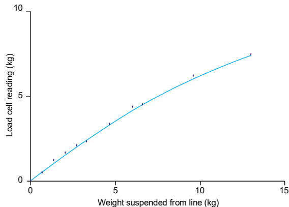
Figure 4. Relationship between line tension and tension meter load cell readings, including fitted line used to calculate line tension.
