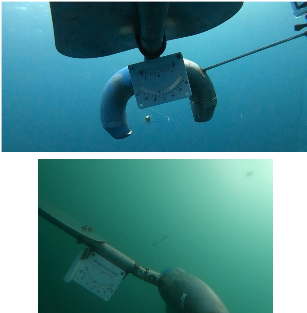
Figure 5. Stills from GoPro camera footage showing view looking aft (top) and view looking sideways (bottom)
