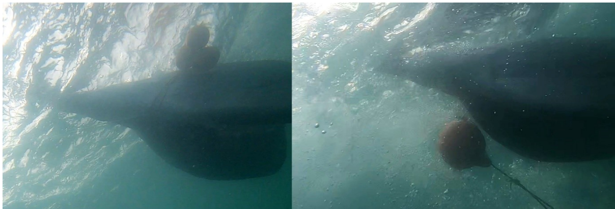
Figure 3d. Stills taken from underwater Go Pro footage showing three egg floats catching on the depressor (left) and a dropper float entering the depressor (right).
