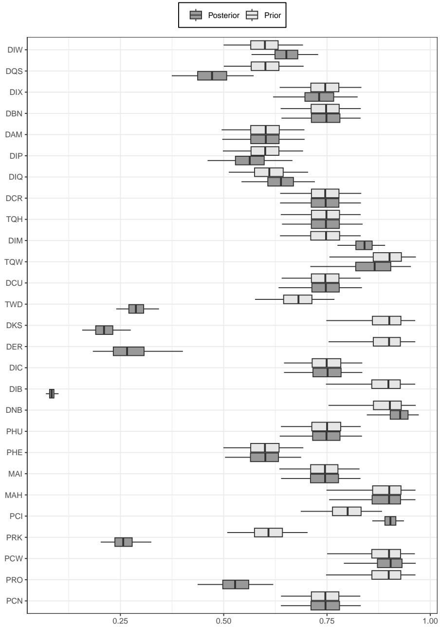
Figure 14: Prior and posterior densities for the proportion bred ( p_b ) for each species (see Table 1). Boxplots show the median, and 75% and 95% posterior quantiles.
