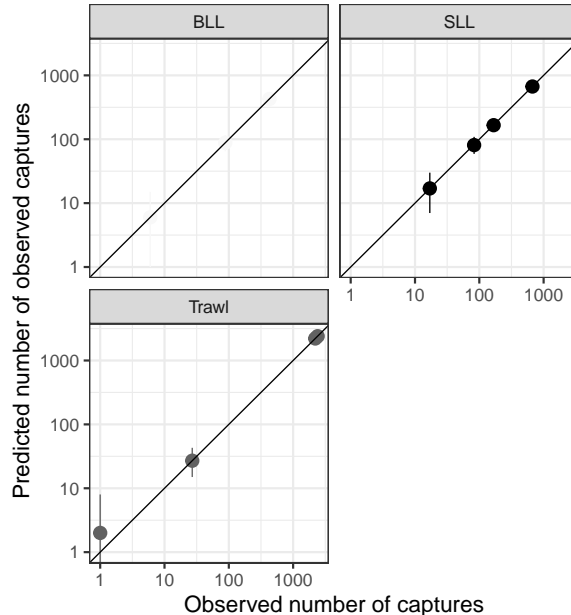
Figure 6: Model fit to the number of observed captures for each fishing method. Zero values are omitted. Captures are summed across species within each species group, between 2006 and 2020, and each point represents a unique combination of species group and fishery group. Median and 95% quantile values are shown.
