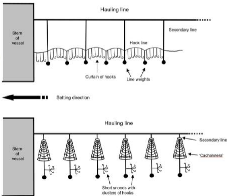
Figure 1. Typical configurations of the traditional Spanish double line system ( top panel ) and Chilean (trotline) system ( bottom panel ) showing differences in gear design and location of weights in relation to hooks. The open-ended secondary/connecting lines (not joined by a continuous hook line) and proximity of weights to hooks of the Chilean system enables hooks to sink rapidly with no lofting in propeller turbulence from the surface close to a vessel stern. Drawings not to scale.
