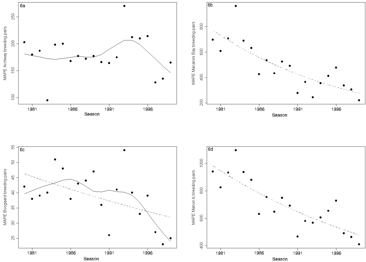
Figures 6a-d. Plots of analyses of Macaroni Penguin population data at a) Archway Bay, Marion I, b) Macaroni Bay, Marion I, c) van den Boogaard, Marion I and d) Marion I study colonies total. The continuous line is the GAM fit to the data, and the dashed line a linear regression fit.
