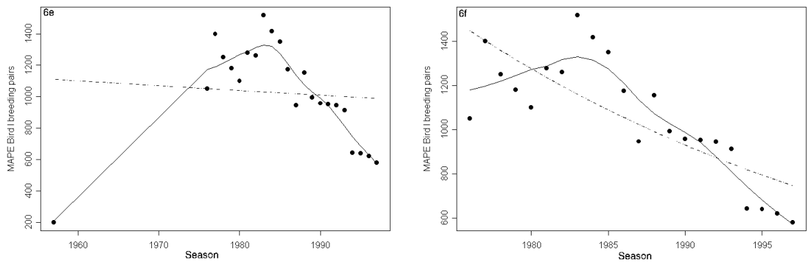
Figures 6e-f. Plots of analyses of Macaroni Penguin population data at e) Bird I and f) Bird I since 1977. The continuous line is the GAM fit to the data, and the dashed line a linear regression fit.
