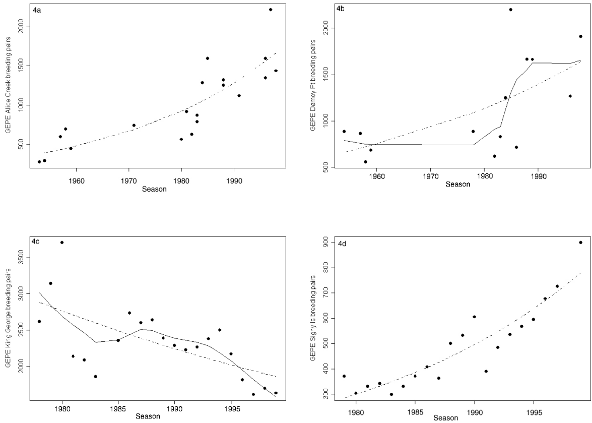
Figures 4a-d. Plots of analyses of Gentoo Penguin population data at four localities in the Antarctic Peninsula: a) Alice Creek (Port Lockroy), b) Damoy Pt (Port Lockroy), c) King George I and d) Signy I. The continuous line is the GAM fit to the data, and the dashed line a linear regression fit.
